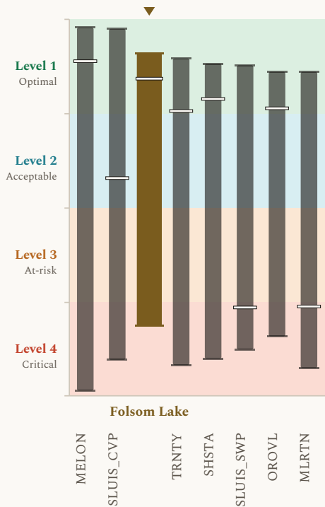
Figure 2. Storage results, presented as modeled outcome levels, across the 8 reservoir storage locations, with Folsom Lake marked. Each column shows the span of modeled results for one reservoir across the COEQWAL library. Ends of a column are the lowest and the highest modeled value at that location across the runs that report it. A short dash across a column is that location’s own baseline (current operations under the historical hydroclimate). This figure uses the same value axis (y-axis) format as Figure 1. Every column uses the same encoding; the column for Folsom Lake, this brief’s subject, is drawn wider, in a distinct color, and marked above. The scale is set out in how to read the values.
