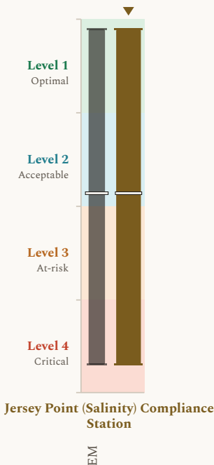
Figure 2. Water quality results, presented as modeled outcome levels, across the 2 freshwater for in-Delta uses locations, with Jersey Point (Salinity) Compliance Station marked. Each column shows the span of modeled results for one Delta compliance station across the COEQWAL library. Ends of a column are the lowest and the highest modeled value at that location across the runs that report it. A short dash across a column is that location's own baseline (current operations under the historical hydroclimate). This figure uses the same value axis (y-axis) format as Figure 1. Every column uses the same encoding; the column for Jersey Point (Salinity) Compliance Station, this brief's subject, is drawn wider, in a distinct color, and marked above. The scale is set out in how to read the values.
