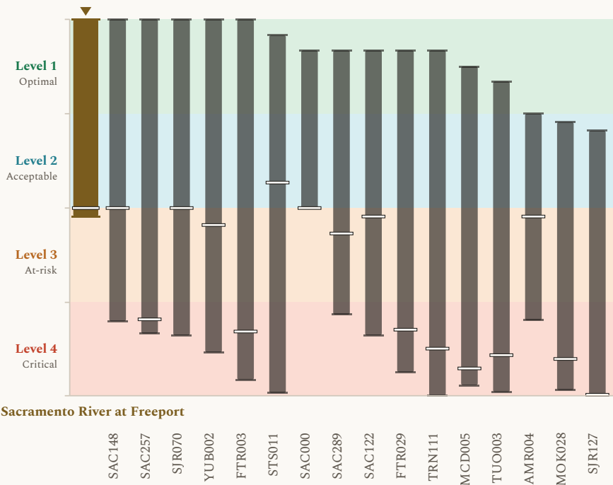
Figure 2. Flow results, presented as modeled outcome levels, across the 17 environmental flows locations, with Sacramento River at Freeport marked. Each column shows the span of modeled results for one river point across the COEQWAL library. Ends of a column are the lowest and the highest modeled value at that location across the runs that report it. A short dash across a column is that location’s own baseline (current operations under the historical hydroclimate). This figure uses the same value axis (y-axis) format as Figure 1. Every column uses the same encoding; the column for Sacramento River at Freeport, this brief’s subject, is drawn wider, in a distinct color, and marked above. The scale is set out in how to read the values.
