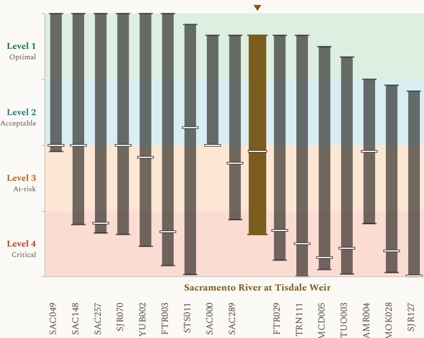
Figure 2. Flow results, presented as modeled outcome levels, across the 17 environmental flows locations, with Sacramento River at Tisdale Weir marked. Each column shows the span of modeled results for one river point across the COEQWAL library. Ends of a column are the lowest and the highest modeled value at that location across the runs that report it. A short dash across a column is that location's own baseline (current operations under the historical hydroclimate). This figure uses the same value axis (y-axis) format as Figure 1. Every column uses the same encoding; the column for Sacramento River at Tisdale Weir, this brief's subject, is drawn wider, in a distinct color, and marked above. The scale is set out in how to read the values.
