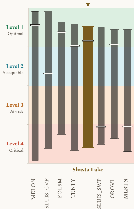
Figure 2. Storage results, presented as modeled outcome levels, across the 8 reservoir storage locations, with Shasta Lake marked. Each column shows the span of modeled results for one reservoir across the COEQWAL library. Ends of a column are the lowest and the highest modeled value at that location across the runs that report it. A short dash across a column is that location’s own baseline (current operations under the historical hydroclimate). This figure uses the same value axis (y-axis) format as Figure 1. Every column uses the same encoding; the column for Shasta Lake, this brief’s subject, is drawn wider, in a distinct color, and marked above. The scale is set out in how to read the values.
