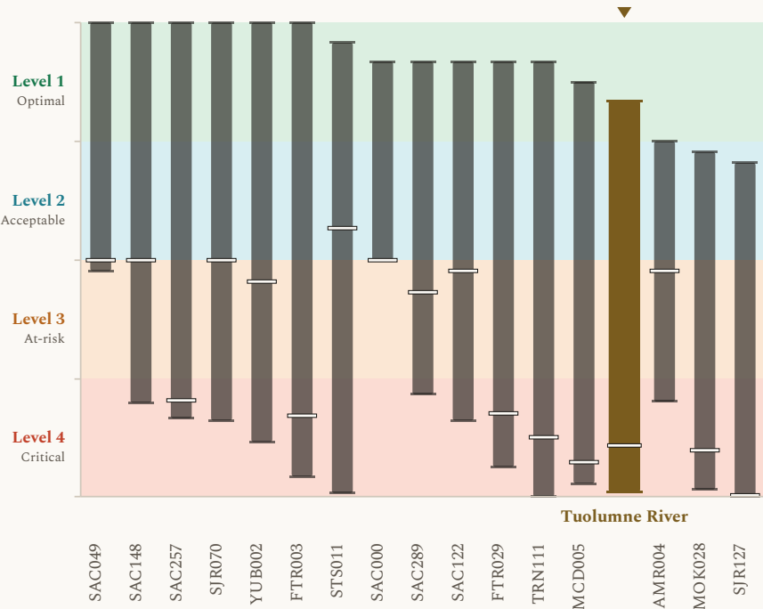
Figure 2. Flow results, presented as modeled outcome levels, across the 17 environmental flows locations, with Tuolumne River marked. Each column shows the span of modeled results for one river point across the COEQWAL library. Ends of a column are the lowest and the highest modeled value at that location across the runs that report it. A short dash across a column is that location’s own baseline (current operations under the historical hydroclimate). This figure uses the same value axis (y-axis) format as Figure 1. Every column uses the same encoding; the column for Tuolumne River, this brief’s subject, is drawn wider, in a distinct color, and marked above. The scale is set out in how to read the values.
