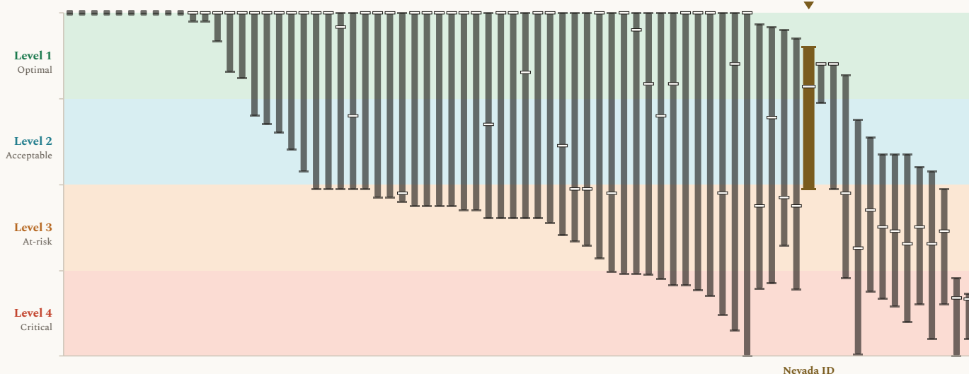
Figure 2. Delivery results, presented as modeled outcome levels, across the 74 community surface water locations, with Nevada ID marked. Each column shows the span of modeled results for one community water system across the COEQWAL library. Ends of a column are the lowest and the highest modeled value at that location across the runs that report it. A short dash across a column is that location's own baseline (current operations under the historical hydroclimate). This figure uses the same value axis (y-axis) format as Figure 1. Every column uses the same encoding; the column for Nevada ID, this brief's subject, is drawn wider, in a distinct color, and marked above. The scale is set out in how to read the values.
