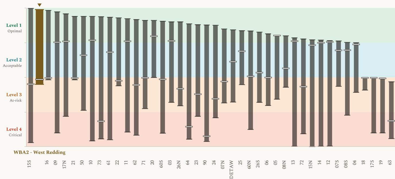
Figure 2. Groundwater storage results, presented as modeled outcome levels, across the 42 groundwater storage locations, with WBA2 - West Redding marked. Each column shows the span of modeled results for one groundwater basin area across the COEQWAL library. Ends of a column are the lowest and the highest modeled value at that location across the runs that report it. A short dash across a column is that location's own baseline (current operations under the historical hydroclimate). This figure uses the same value axis (y-axis) format as Figure 1. Every column uses the same encoding; the column for WBA2 - West Redding, this brief's subject, is drawn wider, in a distinct color, and marked above. The scale is set out in how to read the values.
