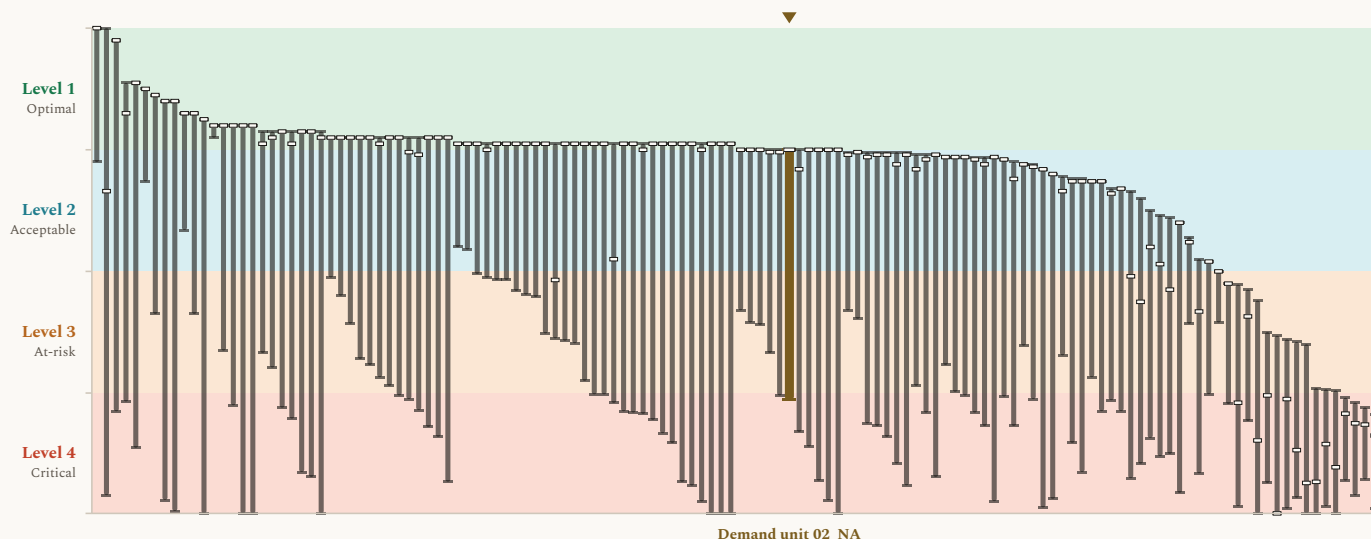
Figure 2. Revenue results, presented as modeled outcome levels, across the 132 agricultural revenue locations, with Demand unit 02_NA marked. Each column shows the span of modeled results for one agricultural water service area across the COEQWAL library. Ends of a column are the lowest and the highest modeled value at that location across the runs that report it. A short dash across a column is that location's own baseline (current operations under the historical hydroclimate). This figure uses the same value axis (y-axis) format as Figure 1. Every column uses the same encoding; the column for Demand unit 02_NA, this brief's subject, is drawn wider, in a distinct color, and marked above. The scale is set out in how to read the values.
