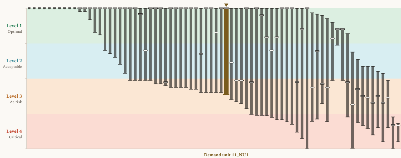
Figure 2. Delivery results, presented as modeled outcome levels, across the 74 community surface water locations, with Demand unit 11_NU1 marked. Each column shows the span of modeled results for one community water system across the COEQWAL library. Ends of a column are the lowest and the highest modeled value at that location across the runs that report it. A short dash across a column is that location's own baseline (current operations under the historical hydroclimate). This figure uses the same value axis (y-axis) format as Figure 1. Every column uses the same encoding; the column for Demand unit 11_NU1, this brief's subject, is drawn wider, in a distinct color, and marked above. The scale is set out in how to read the values.
