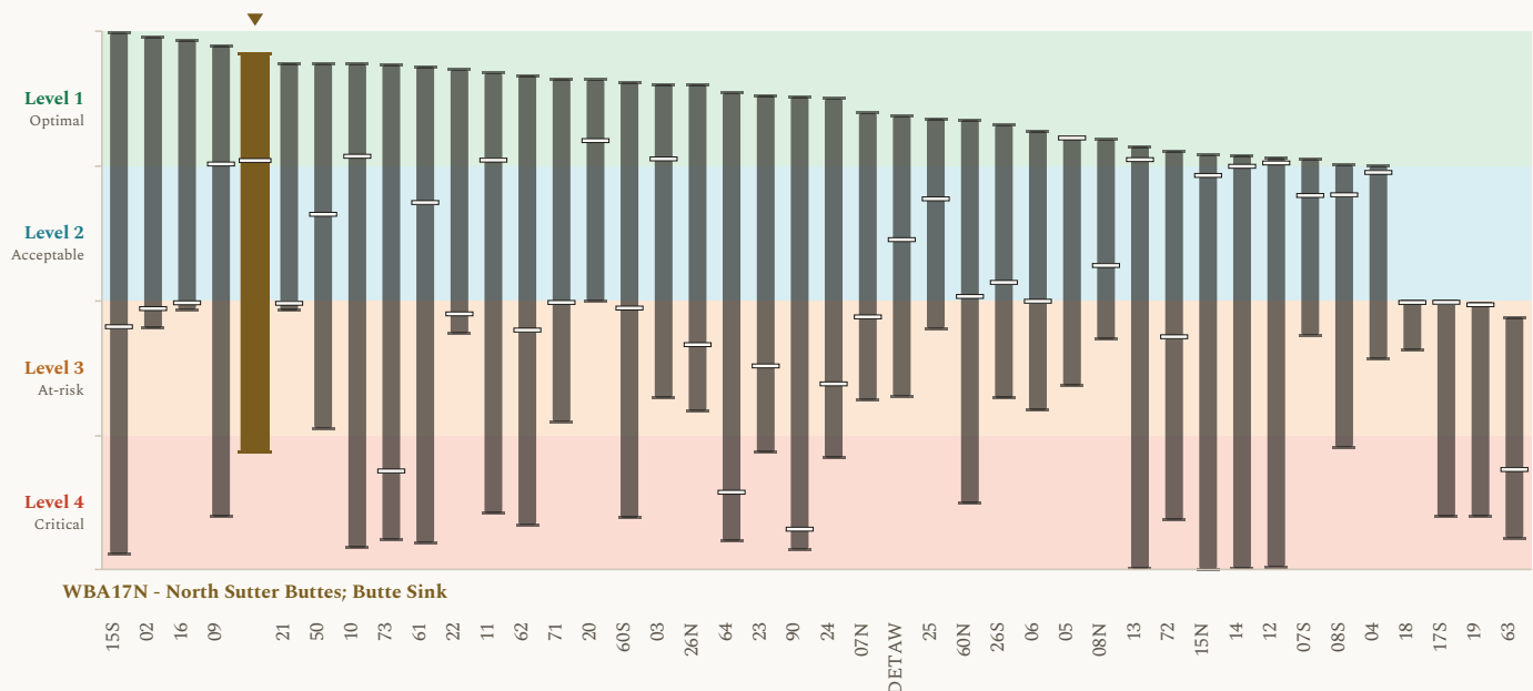
Figure 2. Groundwater storage results, presented as modeled outcome levels, across the 42 groundwater storage locations, with WBA17N - North Sutter Buttes; Butte Sink marked. Each column shows the span of modeled results for one groundwater basin area across the COEQWAL library. Ends of a column are the lowest and the highest modeled value at that location across the runs that report it. A short dash across a column is that location's own baseline (current operations under the historical hydroclimate). This figure uses the same value axis (y-axis) format as Figure 1. Every column uses the same encoding; the column for WBA17N - North Sutter Buttes; Butte Sink, this brief's subject, is drawn wider, in a distinct color, and marked above. The scale is set out in how to read the values.
