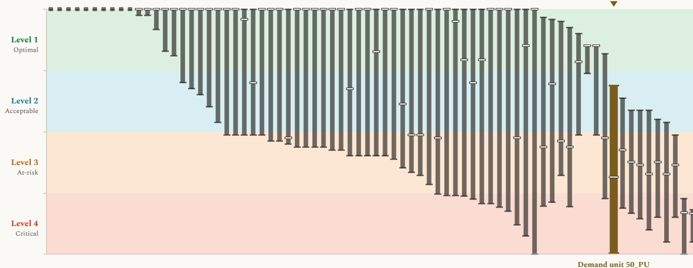
Figure 2. Delivery results, presented as modeled outcome levels, across the 74 community surface water locations, with Demand unit 50_PU marked. Each column shows the span of modeled results for one community water system across the COEQWAL library. Ends of a column are the lowest and the highest modeled value at that location across the runs that report it. A short dash across a column is that location's own baseline (current operations under the historical hydroclimate). This figure uses the same value axis (y-axis) format as Figure 1. Every column uses the same encoding; the column for Demand unit 50_PU, this brief's subject, is drawn wider, in a distinct color, and marked above. The scale is set out in how to read the values.
