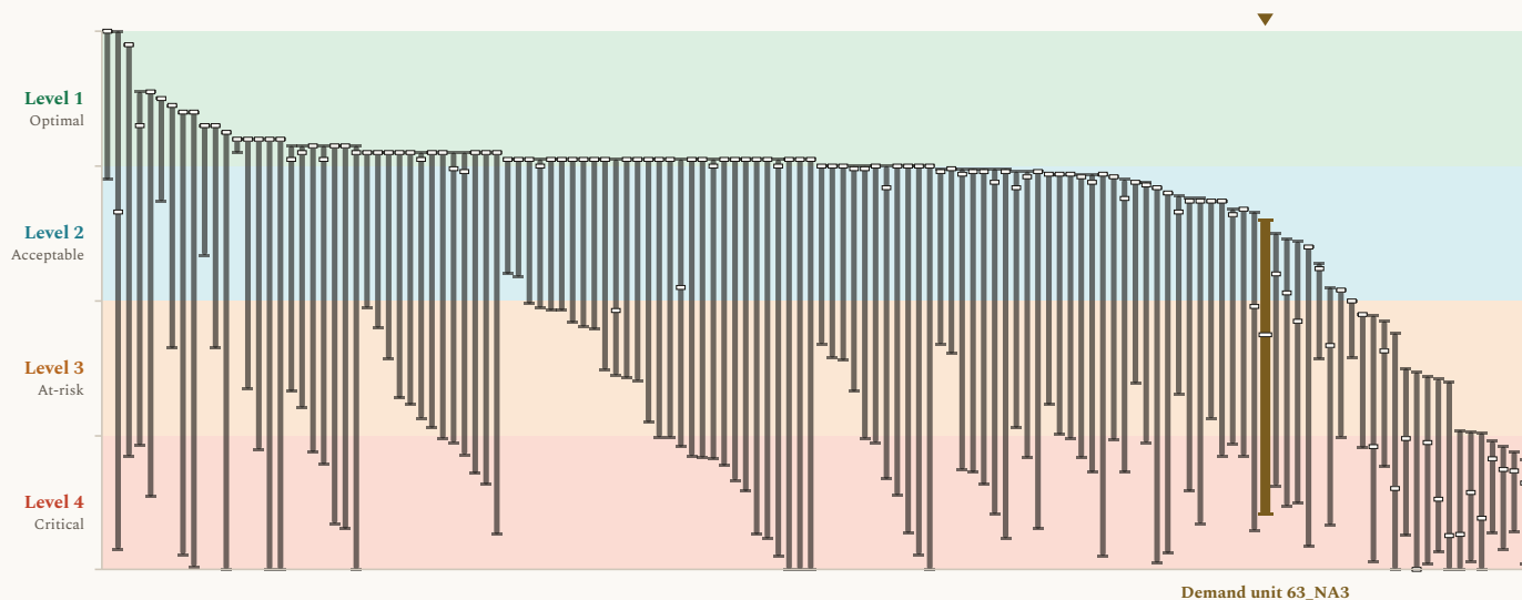
Figure 2. Revenue results, presented as modeled outcome levels, across the 132 agricultural revenue locations, with Demand unit 63_NA3 marked. Each column shows the span of modeled results for one agricultural water service area across the COEQWAL library. Ends of a column are the lowest and the highest modeled value at that location across the runs that report it. A short dash across a column is that location's own baseline (current operations under the historical hydroclimate). This figure uses the same value axis (y-axis) format as Figure 1. Every column uses the same encoding; the column for Demand unit 63_NA3, this brief's subject, is drawn wider, in a distinct color, and marked above. The scale is set out in how to read the values.
