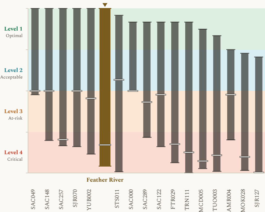
Figure 2. Flow results, presented as modeled outcome levels, across the 17 environmental flows locations, with Feather River marked. Each column shows the span of modeled results for one river point across the COEQWAL library. Ends of a column are the lowest and the highest modeled value at that location across the runs that report it. A short dash across a column is that location’s own baseline (current operations under the historical hydroclimate). This figure uses the same value axis (y-axis) format as Figure 1. Every column uses the same encoding; the column for Feather River, this brief’s subject, is drawn wider, in a distinct color, and marked above. The scale is set out in how to read the values.
