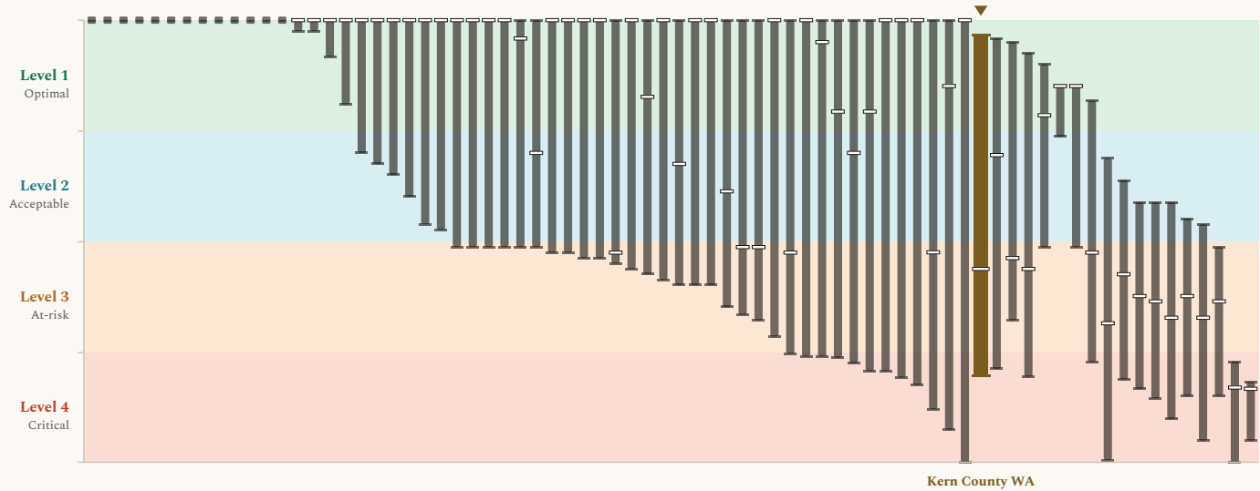
Figure 2. Delivery results, presented as modeled outcome levels, across the 74 community surface water locations, with Kern County WA marked. Each column shows the span of modeled results for one community water system across the COEQWAL library. Ends of a column are the lowest and the highest modeled value at that location across the runs that report it. A short dash across a column is that location's own baseline (current operations under the historical hydroclimate). This figure uses the same value axis (y-axis) format as Figure 1. Every column uses the same encoding; the column for Kern County WA, this brief's subject, is drawn wider, in a distinct color, and marked above. The scale is set out in how to read the values.
