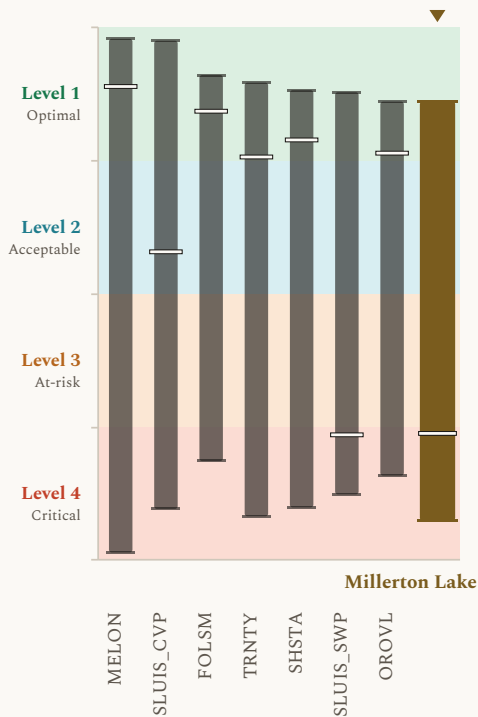
Figure 2. Storage results, presented as modeled outcome levels, across the 8 reservoir storage locations, with Millerton Lake marked. Each column shows the span of modeled results for one reservoir across the COEQWAL library. Ends of a column are the lowest and the highest modeled value at that location across the runs that report it. A short dash across a column is that location’s own baseline (current operations under the historical hydroclimate). This figure uses the same value axis (y-axis) format as Figure 1. Every column uses the same encoding; the column for Millerton Lake, this brief’s subject, is drawn wider, in a distinct color, and marked above. The scale is set out in how to read the values.
