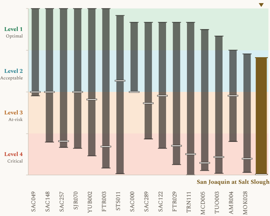
Figure 2. Flow results, presented as modeled outcome levels, across the 17 environmental flows locations, with San Joaquin at Salt Slough marked. Each column shows the span of modeled results for one river point across the COEQWAL library. Ends of a column are the lowest and the highest modeled value at that location across the runs that report it. A short dash across a column is that location’s own baseline (current operations under the historical hydroclimate). This figure uses the same value axis (y-axis) format as Figure 1. Every column uses the same encoding; the column for San Joaquin at Salt Slough, this brief’s subject, is drawn wider, in a distinct color, and marked above. The scale is set out in how to read the values.
