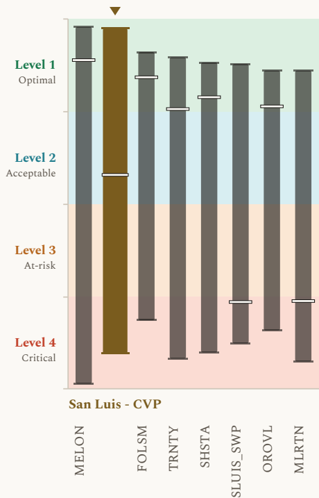
Figure 2. Storage results, presented as modeled outcome levels, across the 8 reservoir storage locations, with San Luis - CVP marked. Each column shows the span of modeled results for one reservoir across the COEQWAL library. Ends of a column are the lowest and the highest modeled value at that location across the runs that report it. A short dash across a column is that location’s own baseline (current operations under the historical hydroclimate). This figure uses the same value axis (y-axis) format as Figure 1. Every column uses the same encoding; the column for San Luis - CVP, this brief’s subject, is drawn wider, in a distinct color, and marked above. The scale is set out in how to read the values.
