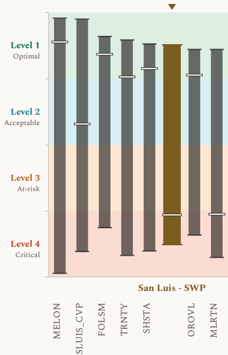
Figure 2. Storage results, presented as modeled outcome levels, across the 8 reservoir storage locations, with San Luis - SWP marked. Each column shows the span of modeled results for one reservoir across the COEQWAL library. Ends of a column are the lowest and the highest modeled value at that location across the runs that report it. A short dash across a column is that location’s own baseline (current operations under the historical hydroclimate). This figure uses the same value axis (y-axis) format as Figure 1. Every column uses the same encoding; the column for San Luis - SWP, this brief’s subject, is drawn wider, in a distinct color, and marked above. The scale is set out in how to read the values.
