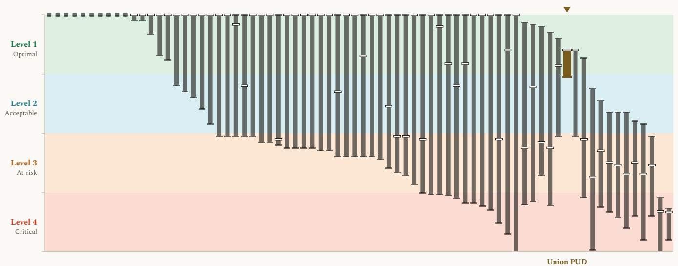
Figure 2. Delivery results, presented as modeled outcome levels, across the 74 community surface water locations, with Union PUD marked. Each column shows the span of modeled results for one community water system across the COEQWAL library. Ends of a column are the lowest and the highest modeled value at that location across the runs that report it. A short dash across a column is that location's own baseline (current operations under the historical hydroclimate). This figure uses the same value axis (y-axis) format as Figure 1. Every column uses the same encoding; the column for Union PUD, this brief's subject, is drawn wider, in a distinct color, and marked above. The scale is set out in how to read the values.
