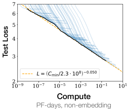
Figure 2: LLM scaling
