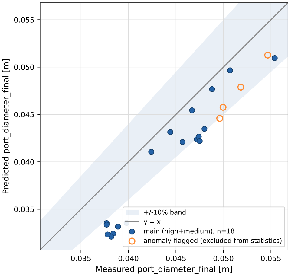
hybrid - port_diameter_final (n=18)
