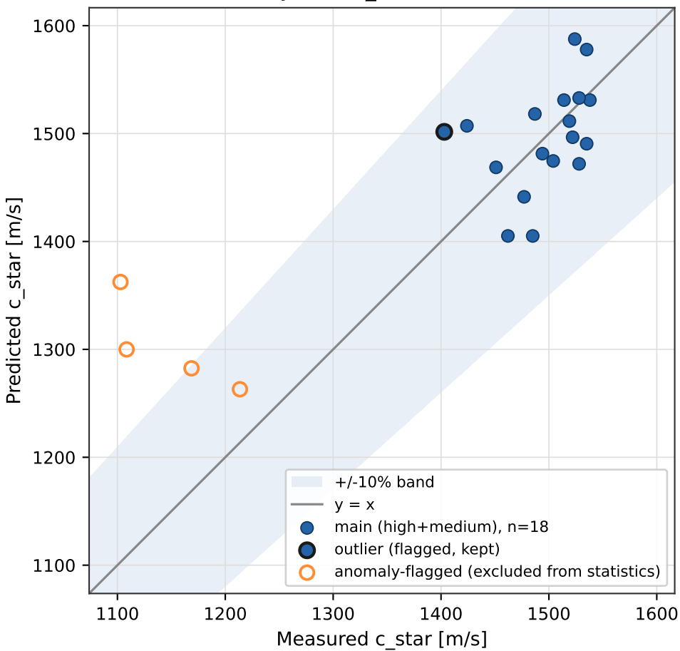
hybrid - c_star (n=18)
