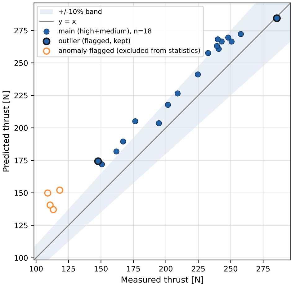
hybrid - thrust (n=18)
