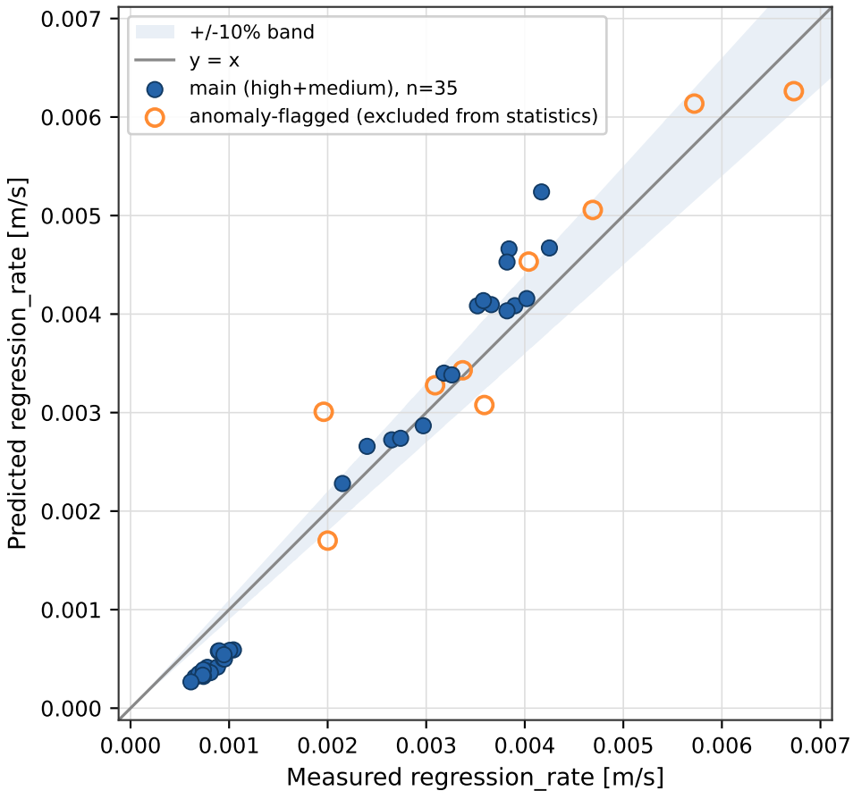
hybrid - regression_rate (n=35)
