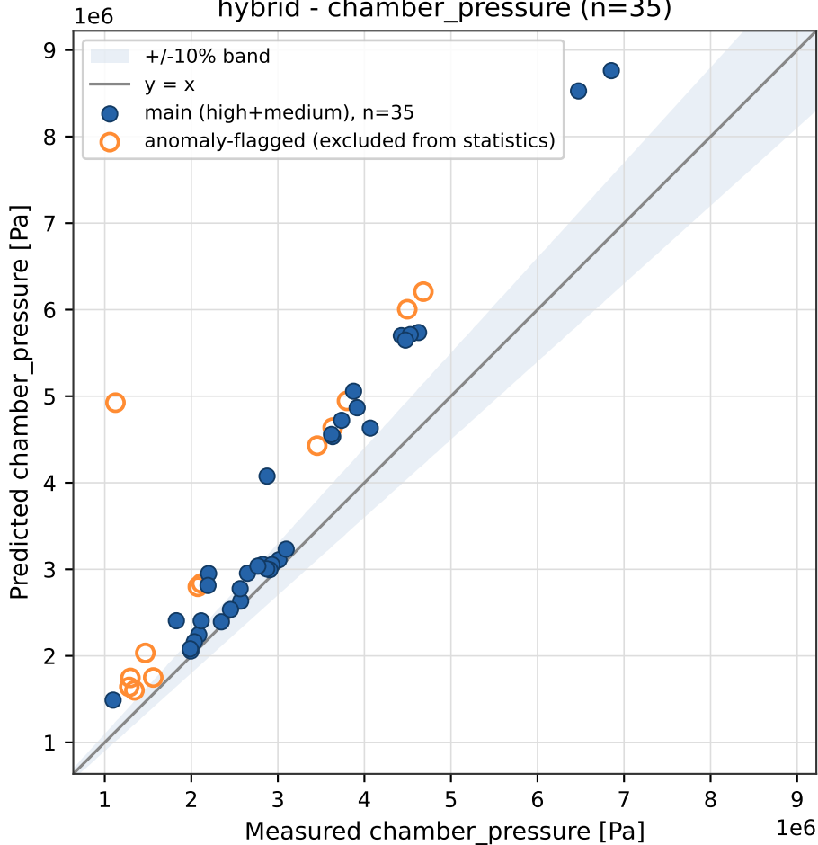
hybrid - chamber_pressure (n=35)
