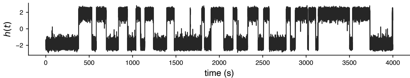
Hidden driver ( \beta = 0.50 )
