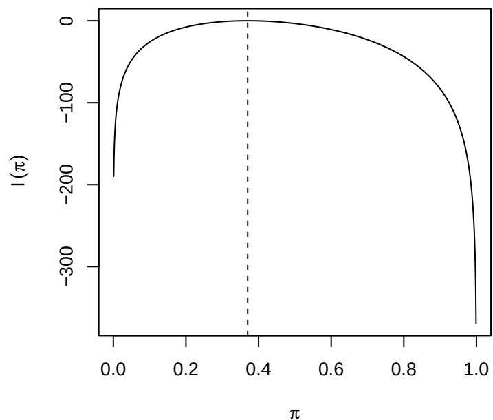
Relative Log-Likelihood
