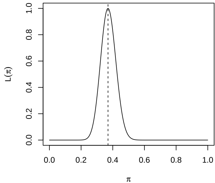
Relative Likelihood
