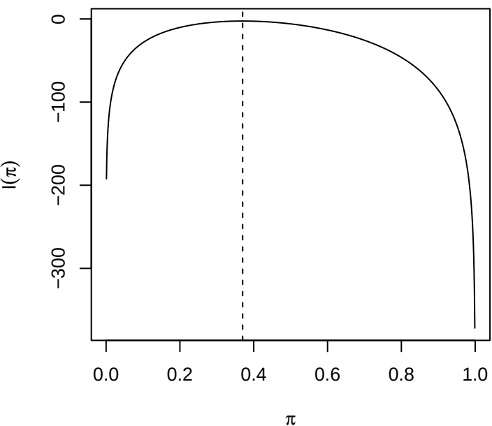
Log-Likelihood
