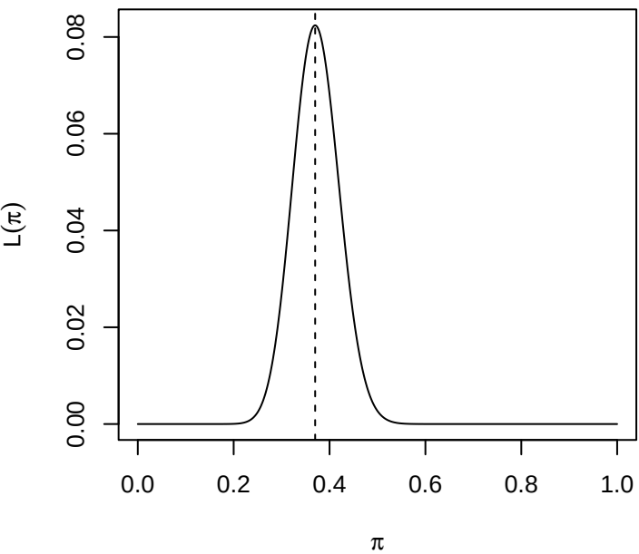
Likelihood
