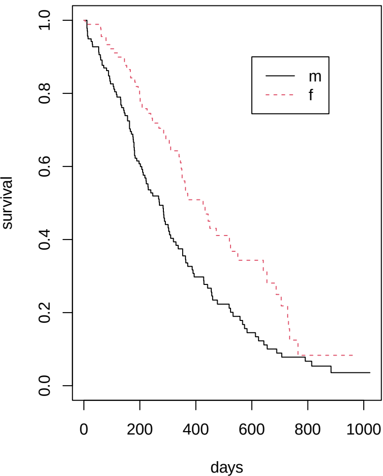
Kaplan–Meier Curves
