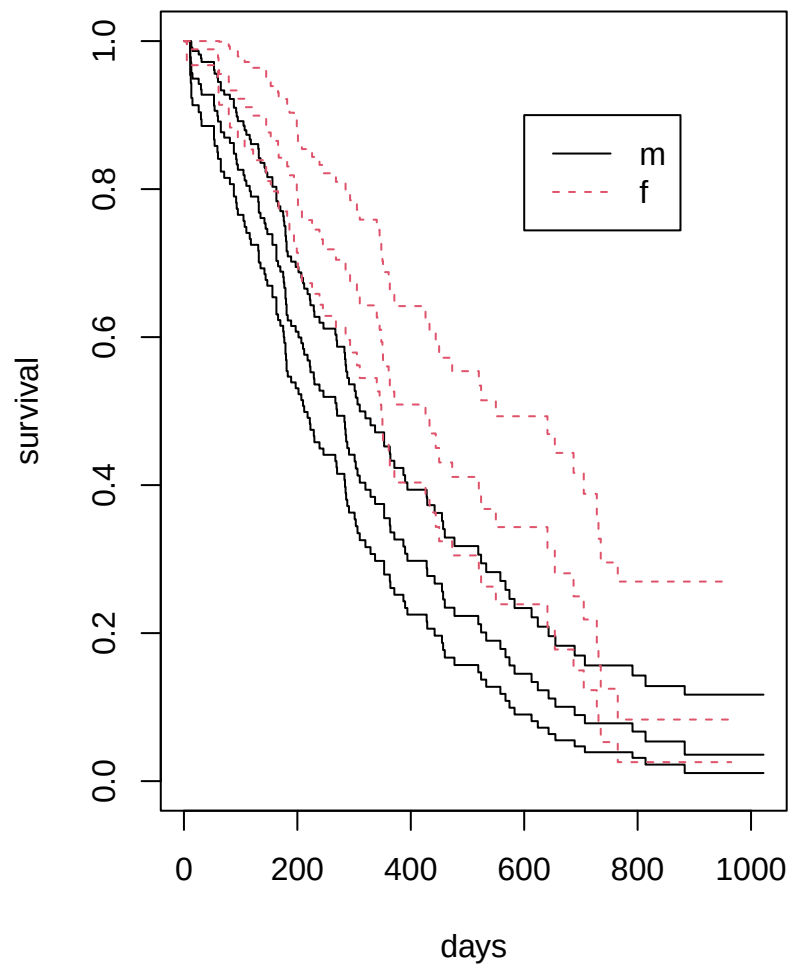
Kaplan–Meier Curves
