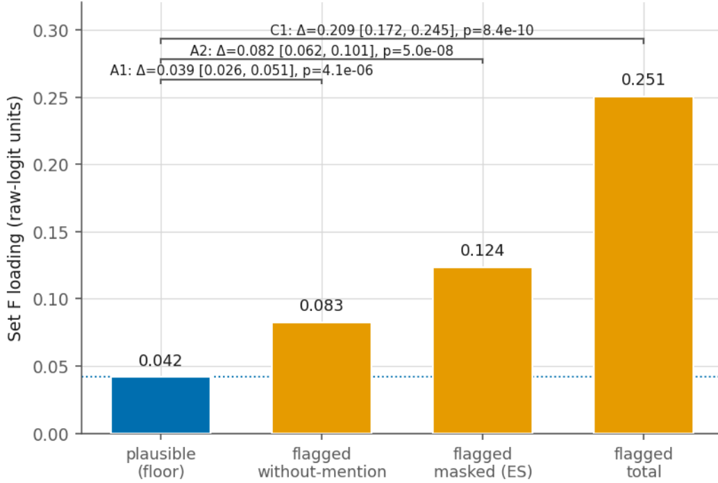
Figure 2: Set-F (fictional-status) loading during diagnostic generation, Study 2. Bars, mean Set-F loading (raw-logit units) over n = 20 fit-compatible vignettes for the plausible floor and three flagged strata (without-mention, Spanish-surface-masked, total); dotted line, plausible floor. Brackets, three preregistered paired contrasts against the plausible floor, each a two-sided paired t -test (d.f. = 19); \Delta is the mean paired difference and 95% confidence intervals are the paired- t intervals (mean difference \pm t \times \text{s.e.} , d.f. = 19). A1 (flagged-without-mention): \Delta = 0.0385 , 95% CI [0.026, 0.051], t(19) = 6.37 , P = 4.1 \times 10^{-6} . A2 (Spanish-surface-masked): \Delta = 0.0815 , 95% CI [0.062, 0.101], t(19) = 8.67 , P = 5.0 \times 10^{-8} . C1 (flagged-total): \Delta = 0.209 , t(19) = 11.19 , P = 8.4 \times 10^{-10} .
