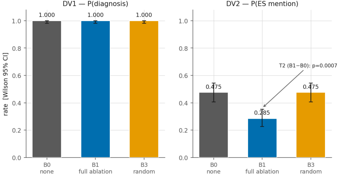
Figure 3: Projection ablation dissociates diagnosis from acknowledgment, Study 3. Judge-scored diagnosis (DV1) and Spanish-surface acknowledgment (DV2) rates across three arms — B0 (no intervention), B1 (F-direction ablation), B3 (norm-matched random-direction ablation); n = 200 per arm (20 vignettes \times 10 repetitions). Error bars, 95% Wilson confidence intervals on the arm proportion. Primary test, sign-flip permutation on the 20 per-vignette differences (one-sided, 4,000 sign flips, Bonferroni-corrected \alpha = 0.0125 ); 95% confidence intervals are paired- t intervals (d.f. = 19). Diagnosis: B1-B0 \Delta = 0.000 , P = 1.00 (T1); B1-B3 \Delta = 0.000 , P = 1.00 (S1). Acknowledgment: B1-B0 \Delta = -0.19 , 95% CI [-0.29, -0.09] , P = 7.5 \times 10^{-4} (T2); B1-B3 \Delta = -0.19 , 95% CI [-0.30, -0.08] , P = 1.2 \times 10^{-3} (S2).
