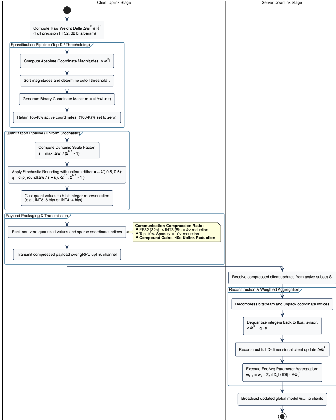
Figure 8.1: Communication Efficiency Pipeline (communication_efficiency.svg), detailing the swimlane pipeline for Top- K sparsification, stochastic quantization, payload packing, and server-side reconstruction.
