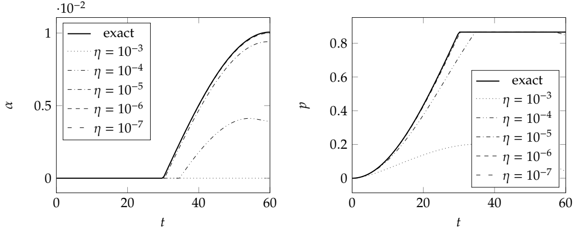
FIGURE 7.2. Comparison between exact and computed values of \alpha and p for some values of \eta . Similar result are found for \lambda . The parameters used are L = 2 , H = 1 , m = 100 , l = 100 , a = \sqrt{2} \sin \phi , b = \sqrt{2} \sin \psi and f_0 = \sqrt{2}c \cos \phi with \phi = 30^\circ , \psi = 5^\circ and c = 0.5 . Moreover the time t ranges in [0, 60] and \epsilon(t) = \frac{1.3 \cdot 10^{-2}}{2} \left[ 1 - \cos \left( \pi \frac{t}{60} \right) \right] .
