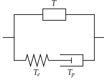
FIGURE 8.1. Rheological model describing the choice of the internal virtual power \tilde{W} . The box in upper branch represents the (generic) macroscopic response. In the lower branch, the spring represents the elastic response and the piston represents the microscopic response. We notice that the microscopic response besides the usual dissipative plastic microforce force can include conservative microforces to model hardening. A more detailed discussion on constitutive relations is in Section 8.1.3.
