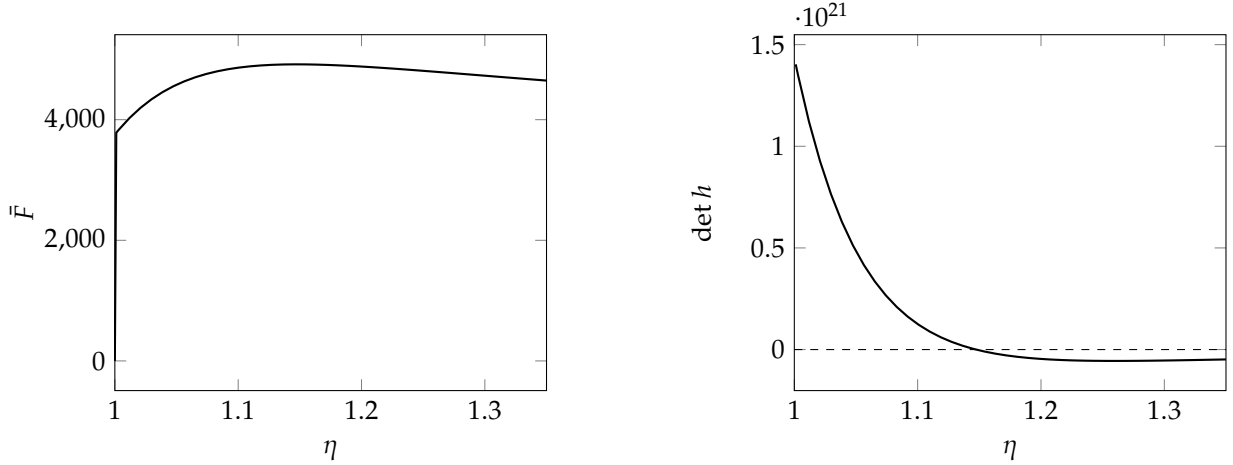
FIGURE 5.3. Graphs of \bar{F} and \det h as functions of the elongation \eta along the trivial solution in the plastic model. Notice that the maximum of \bar{F} is reached when h vanishes at \eta_m = 1.1474 .
