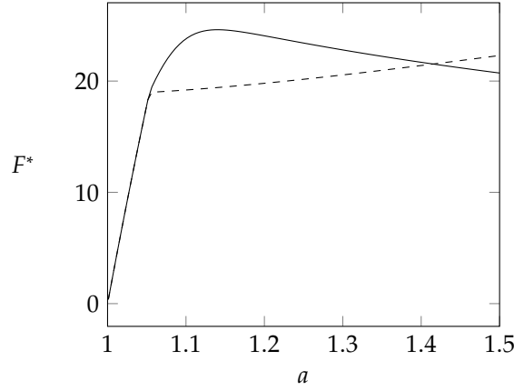
FIGURE 5.3. Graphs of F^* and \lambda as functions of the elongation a along the homogeneous solution in the plastic model. The solid line is referred to H in (ii) and the dashed line to H in (i).
