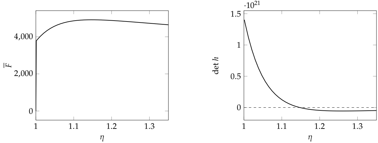
FIGURE 5.3. Graphs of \bar{F} and \det h as functions of the elongation \eta along the trivial solution in the plastic model. Notice that the maximum of \bar{F} is reached when h vanishes at \eta = 1.1474 .
