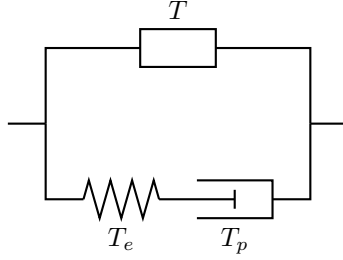
FIGURE 1. Rheological model describing the choice of the internal virtual power \tilde{\mathcal{W}} . The box in upper branch represents the (generic) macroscopic response. In the lower branch, the spring represents the elastic response and the piston represents the microscopic response. We notice that the microscopic response besides the usual dissipative plastic microforce force can include conservative microforces to model hardening. A more detailed discussion on constitutive relations is in Section 1.3.
