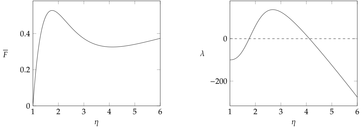
FIGURE 5.2. Graphs of \bar{F} and \lambda as functions of the imposed elongation \eta for the homogeneous deformation in the purely elastic model with the choice of the value of the parameters in 5.21.
