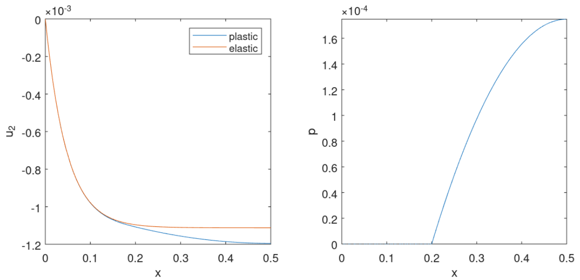
FIGURE 2. Plot of u_2 (left) and p (right) for \epsilon = 0.3 .
