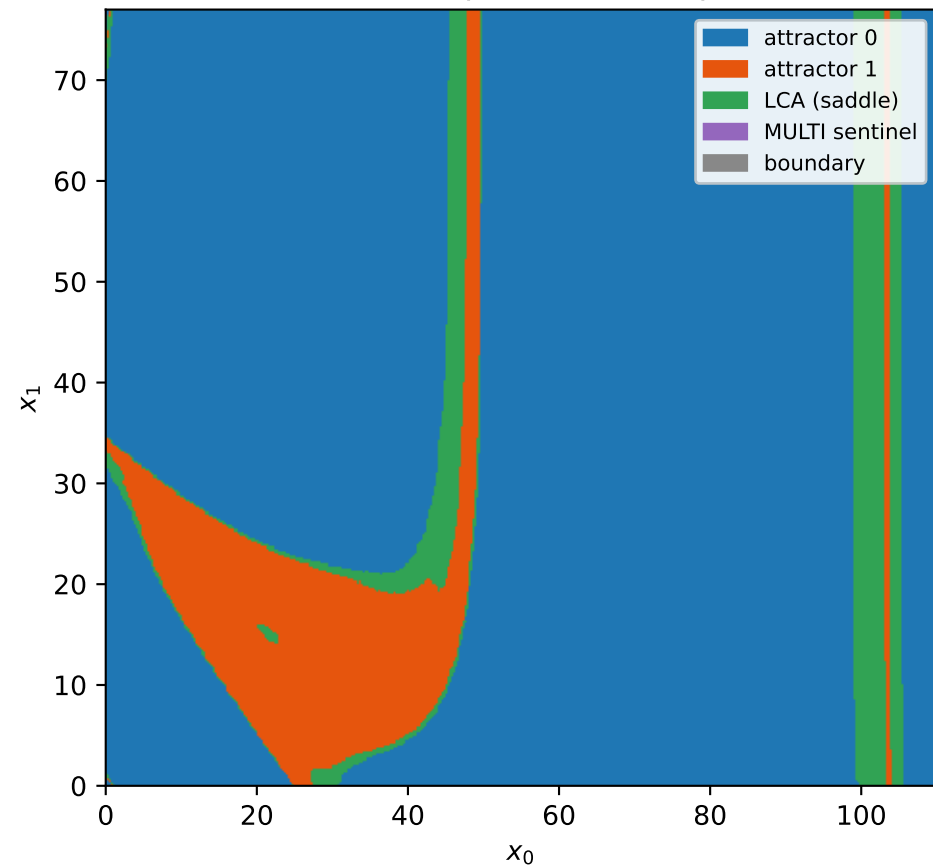
Mode 3: explicit LCA collapse
