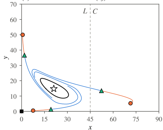
(a) invariant sets and W^u(s_3)
