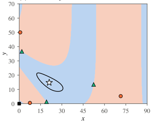
(b) basins of a_3 and \Gamma
