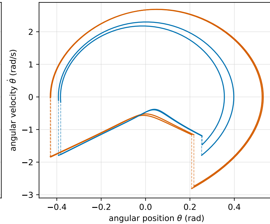
(c) Period 4 | \phi = 5.00^\circ
