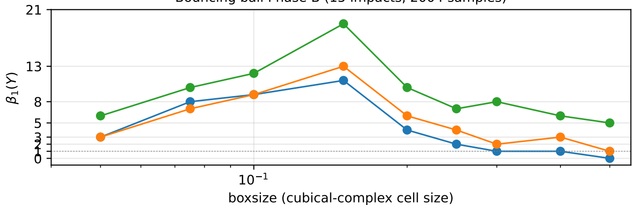
Bouncing ball Phase-B (15 impacts, 2004 samples)
