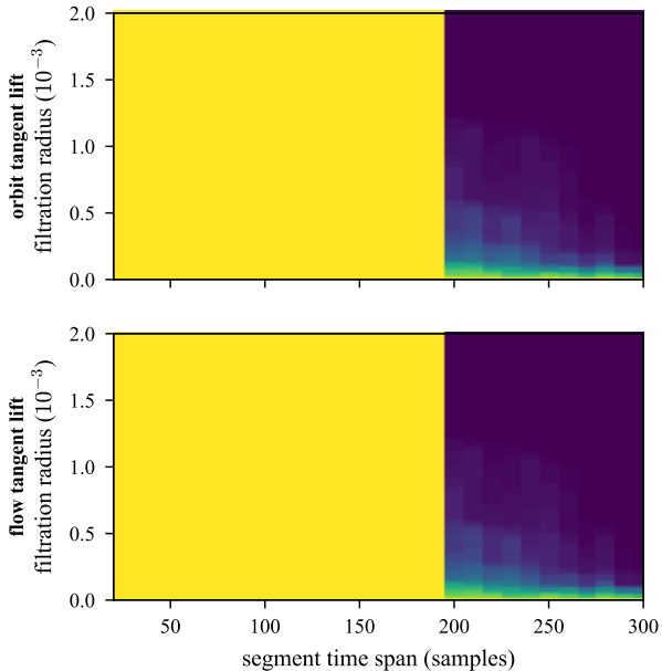
rank 0
