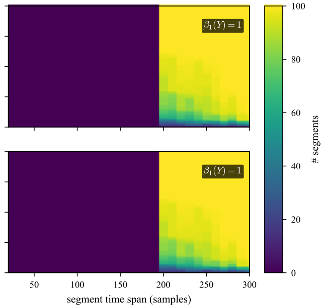
rank 1
