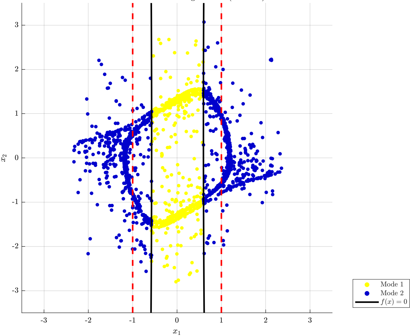
Identified vs True Switching Surface (SPS LC)
