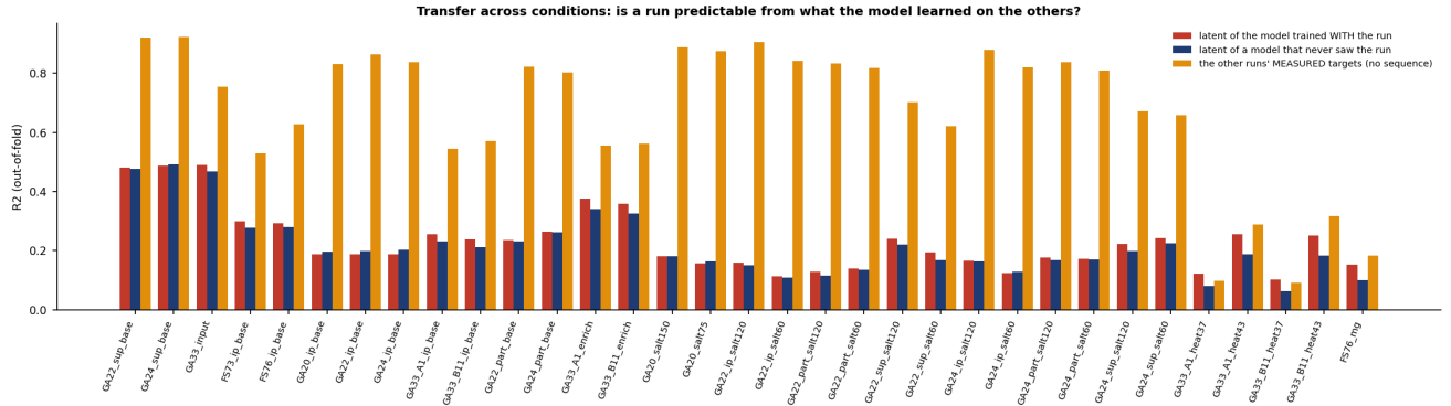
Figure 5: For each target: read-out from the latent of the model trained with the run (red), from a trunk that never saw the run (blue), and, for scale, the prediction from the other runs' MEASURED targets with no sequence (orange).
