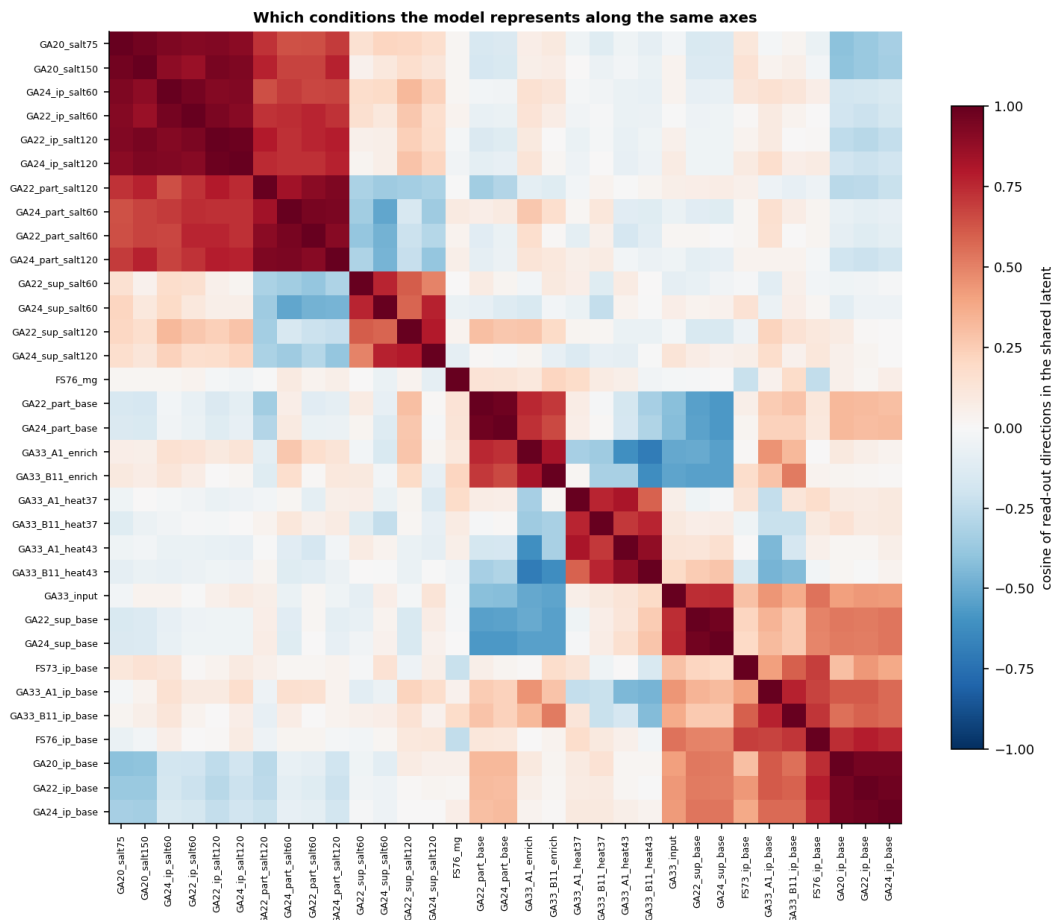
Figure 6: Cosine between targets' read-out directions in the shared latent, clustered.
