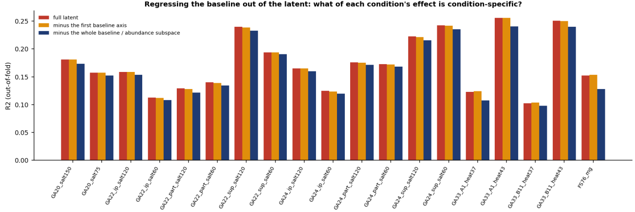
Figure 7: Effect targets read from the full latent, from the latent minus its first baseline axis, and minus the whole baseline / abundance subspace.
