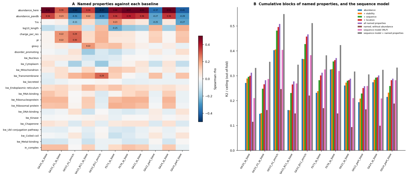
Figure 4: A: Spearman rho of each named property with each baseline. B: out-of-fold R^2 / ceiling as property blocks are added, the sequence MLP alone, and the two combined.
