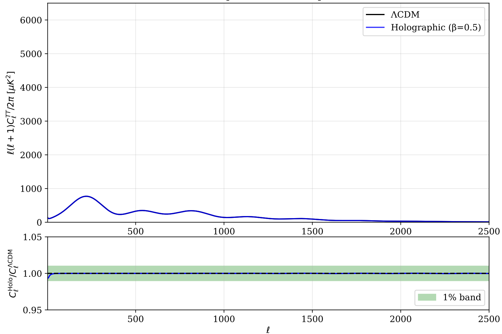
CMB Temperature Power Spectrum
