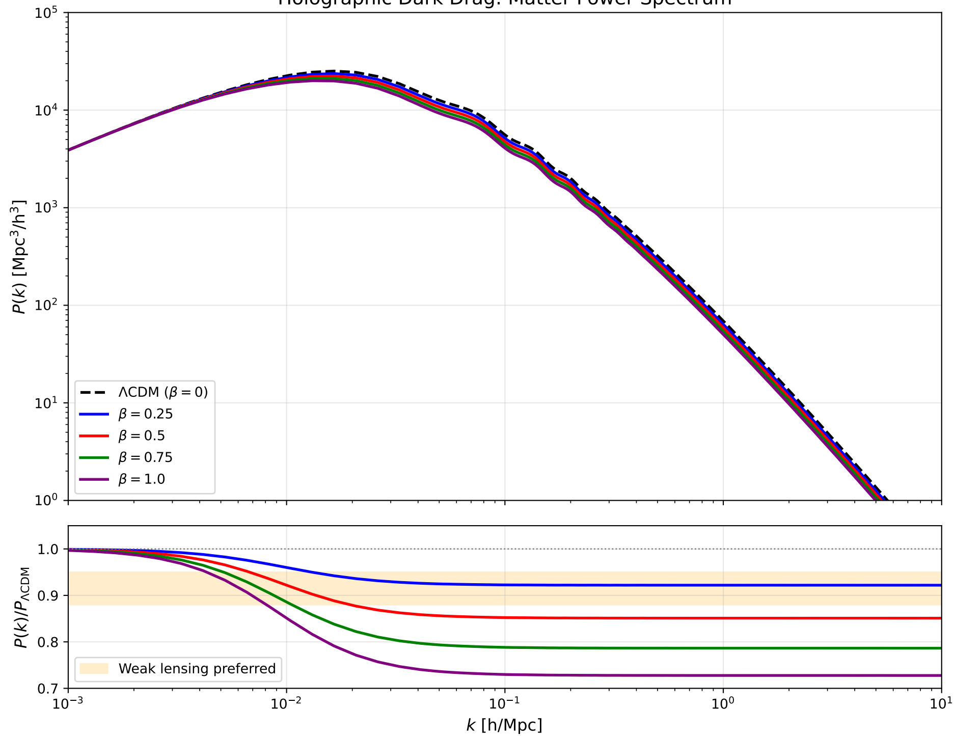
Holographic Dark Drag: Matter Power Spectrum
