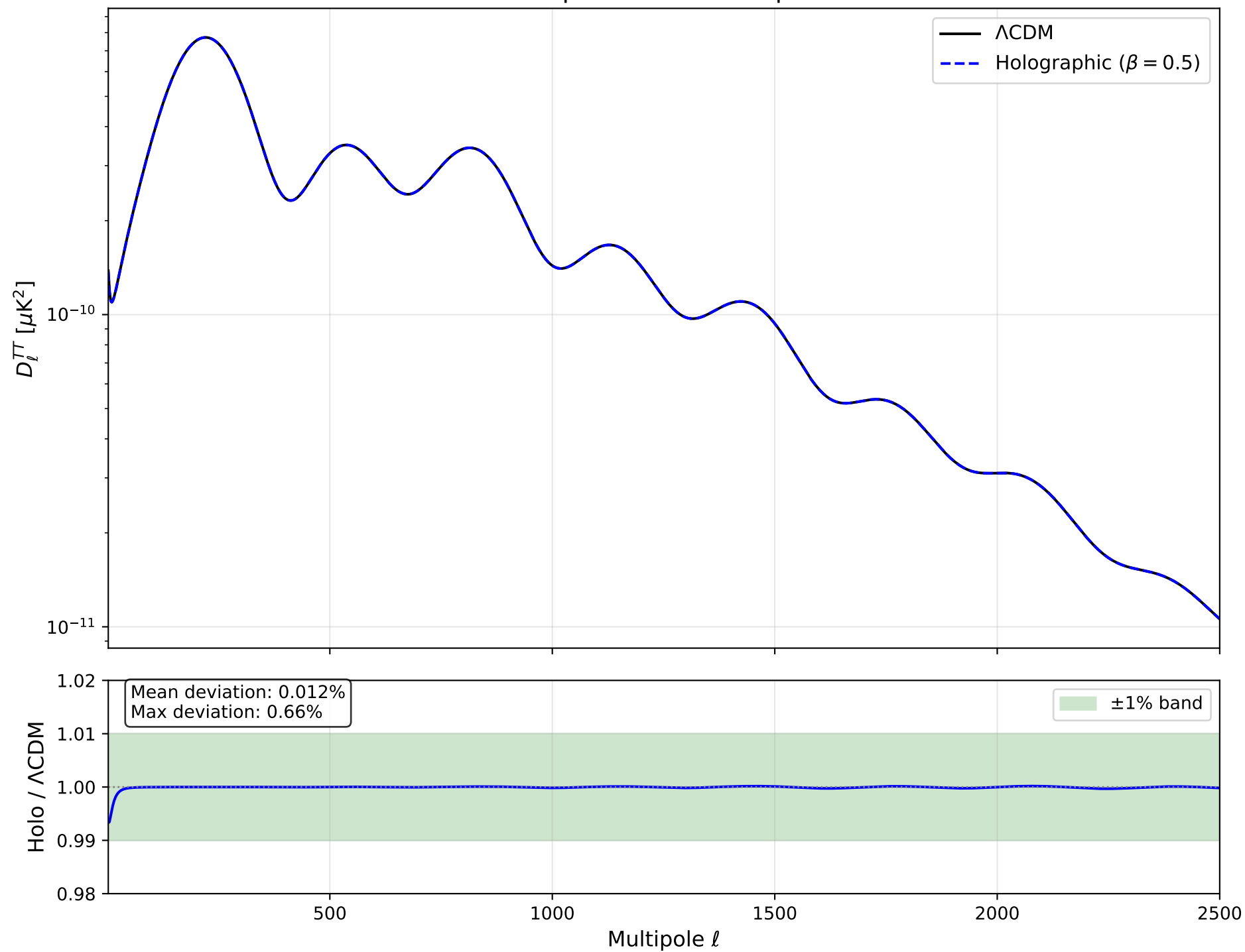
CMB Temperature Power Spectrum
