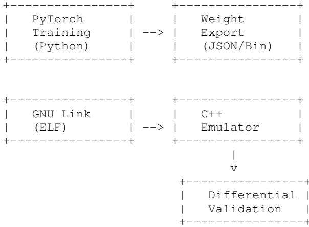
Fig. 1. End-to-End Neural Execution Pipeline. The pipeline ensures bit-exact parity between software and hardware backends through automated differential tests.
