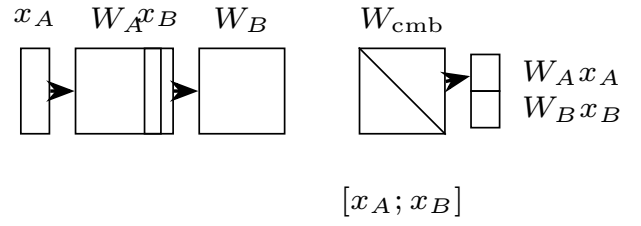
Fig. 7. Block-Diagonal Model Composition. Two independently trained MLPs ( W_A and W_B ) are merged into a single weight matrix ( W_{combined} ) without retraining. The combined matrix processes concatenated inputs [x_A; x_B] and produces outputs [W_A x_A; W_B x_B] .
