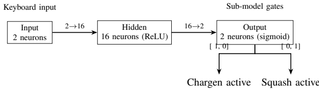
Fig. 9. Router MLP Architecture. The 2 \rightarrow 16 \rightarrow 2 MLP acts as a learned scheduler, using sigmoid outputs to gate sub-models (e.g., chargen, squash) based on keyboard input. The architecture ensures deterministic gating behavior and process scheduling semantics.
