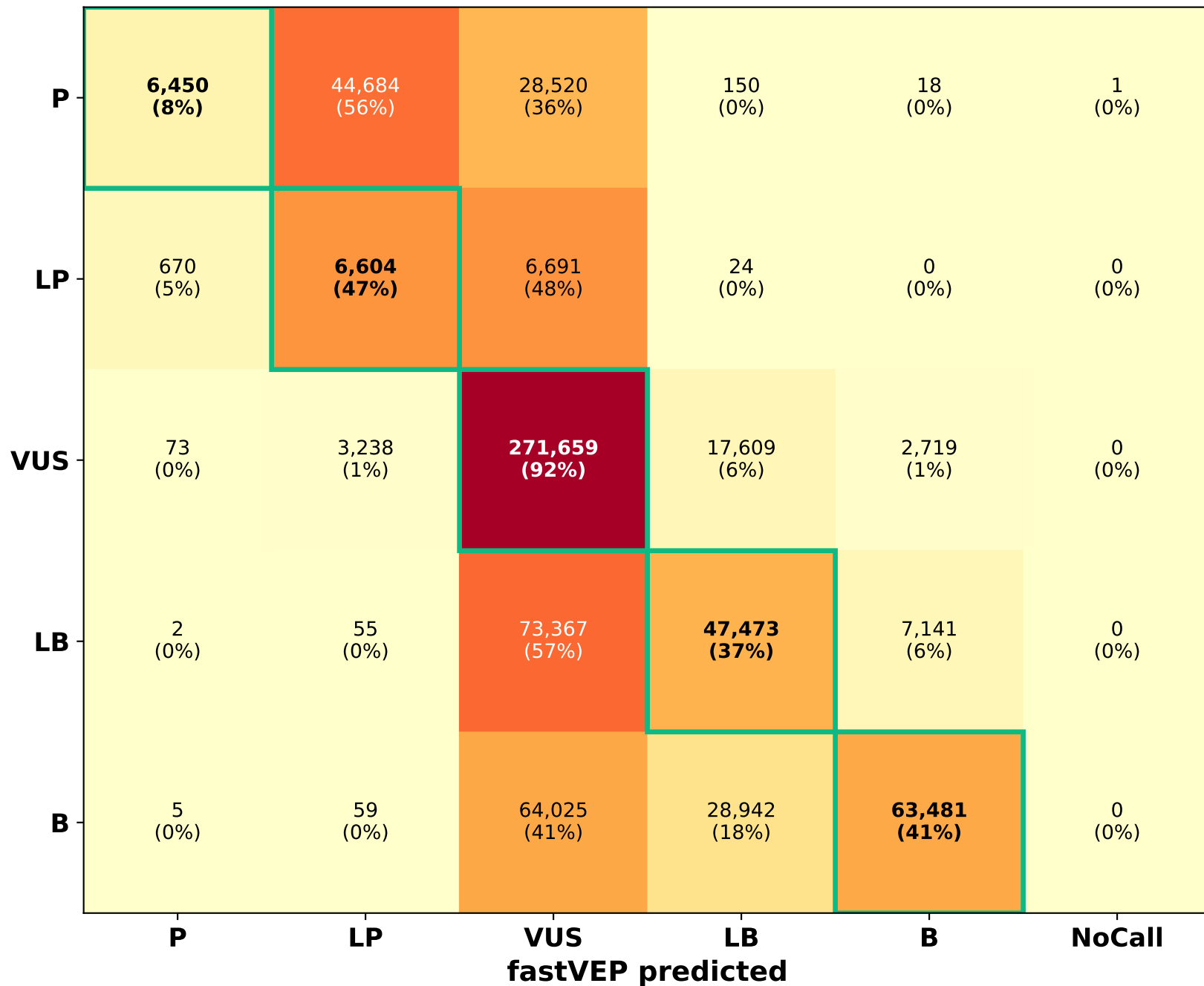
ACMG concordance matrix (row-normalised %)
