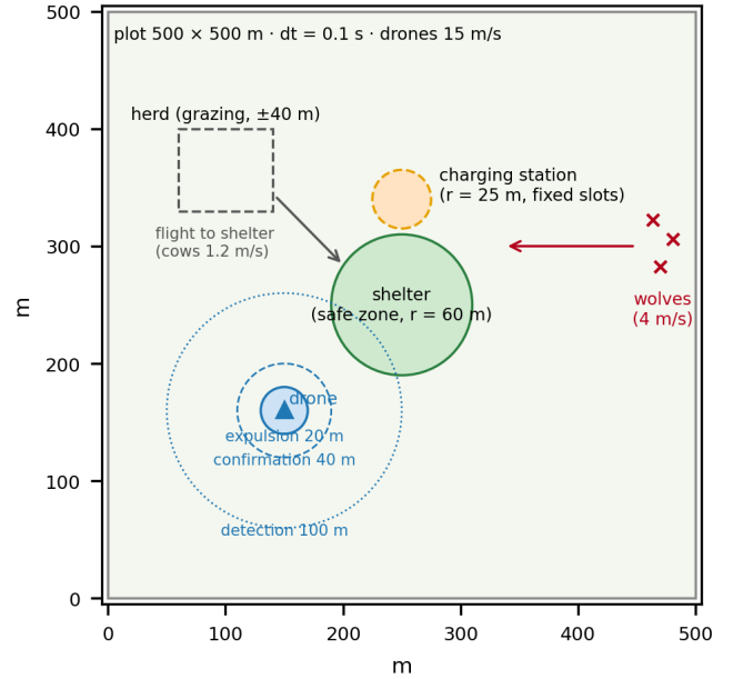
Fig. 2. Environment schematic: 500 \times 500 m field with central shelter, charging station, herd, and the drone’s perception/deterrence radii (expulsion 20 m, confirmation 40 m, detection 100 m). Positions are illustrative.
