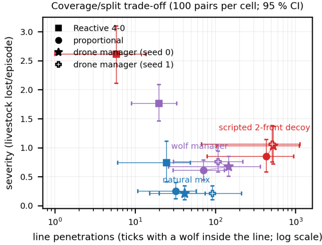
Fig. 5. Coverage/splitting trade-off: line penetrations versus severity, by defense and attacker type. Splitting buys the second front at the price of thinning the first.
