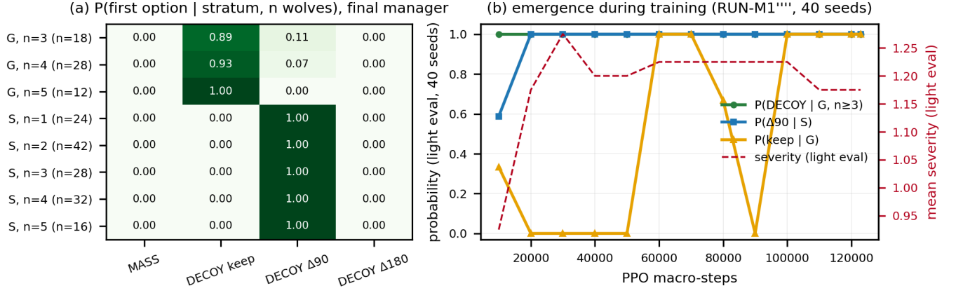
Fig. 4. (a) Final policy of the attacking manager: probability of the first option by spawn stratum and wolf count ( keep under grouped spawns 0.89–1.00; \Delta 90 under dispersed ones 1.00 for all n ). (b) Emergence curve during training (light evaluation, 40 seeds).
