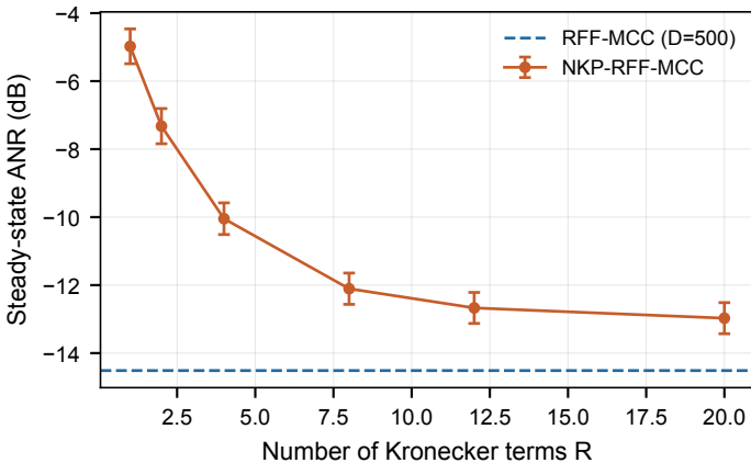
Logistic-chaotic reference, \mu = 0.2
