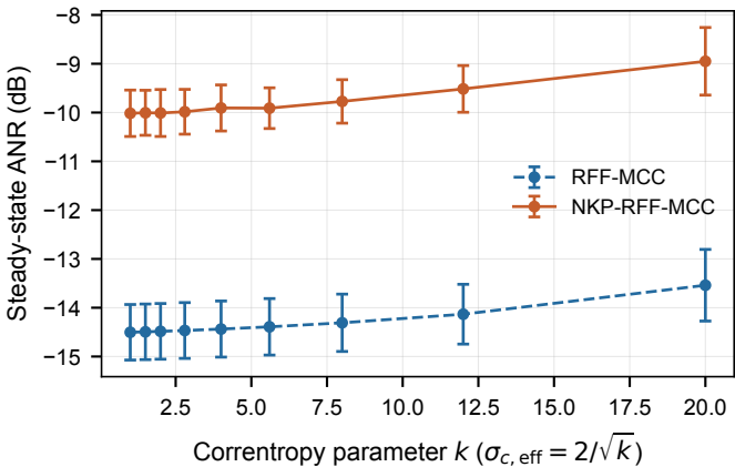
Logistic-chaotic reference, \mu = 0.2
