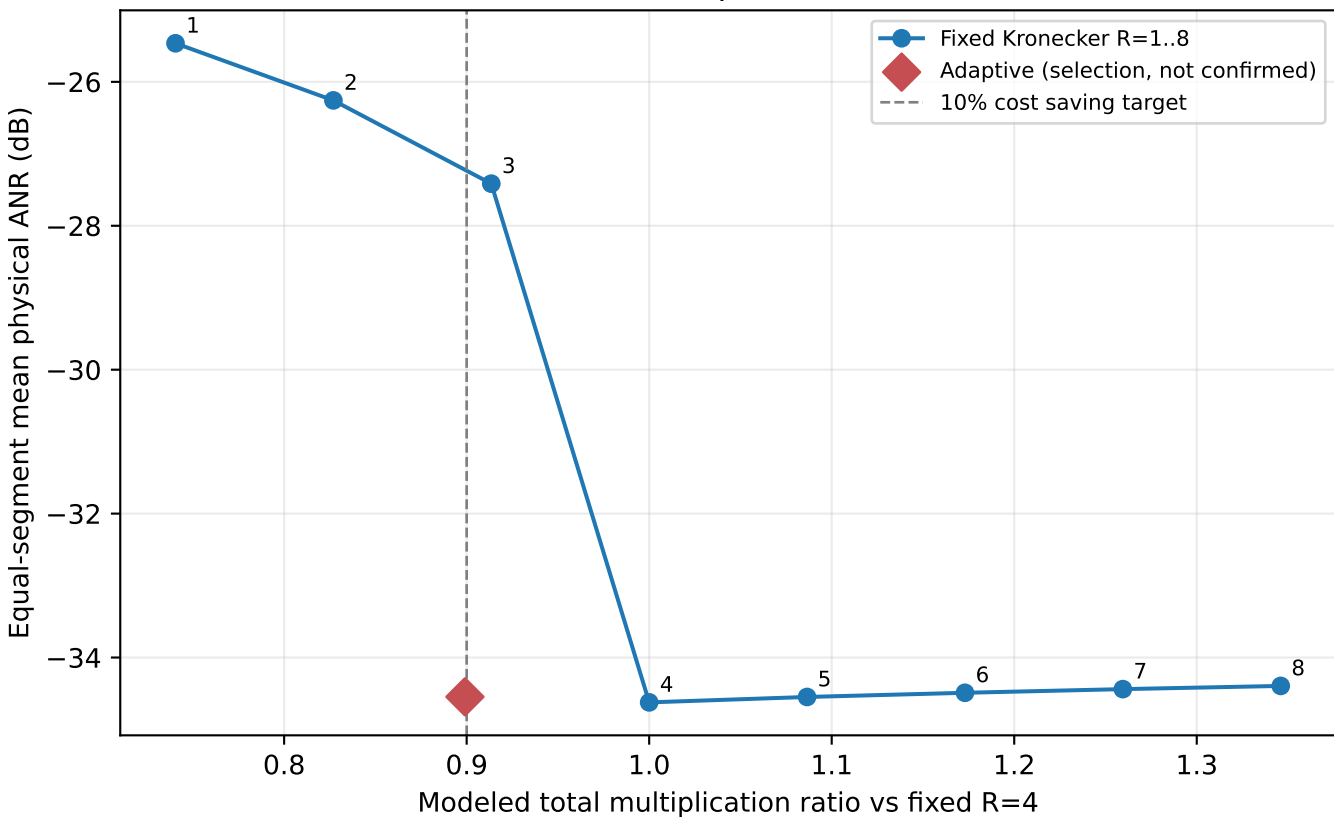
E1 known-rank teacher: independent selection set (8 runs)
